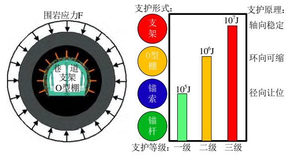
图 22 三级支护原理示意 Fig. 22 Schematic principle of three-stage support
