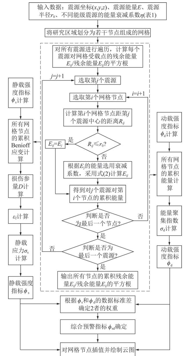
图12 基于震动波能量衰减特性的冲击危险预测方法计算流程 Fig.12 Calculation flow chart of coal burst prediction method based on energy attenuation characteristics of shock waves
