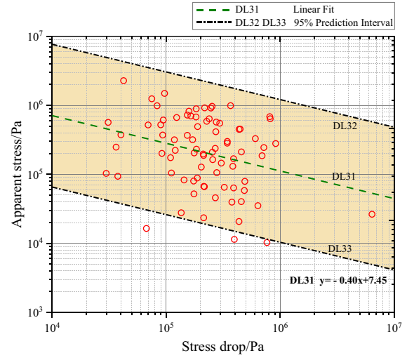
Figure 9. Relation map of stress drop and apparent stress of coal burst events.
