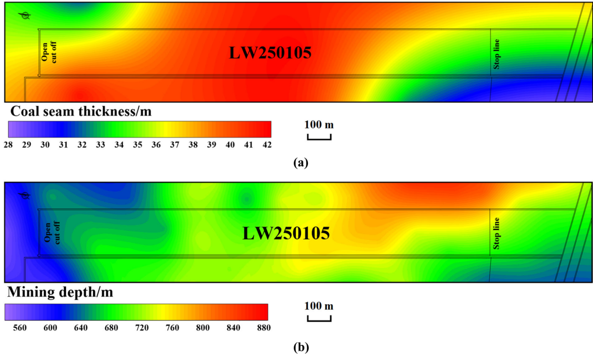
Figure 2. (a) Contours of coal seam thickness in LW250105. (b) Contours of mining depth in LW250105.
