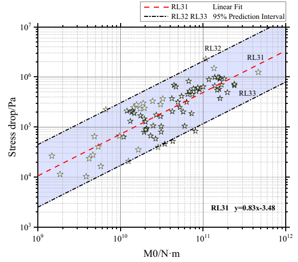
Figure 12. Relation of scalar seismic moment and stress drop of coal burst events.
